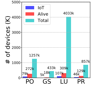
(d) # of IoT devices observed from each RESIP service provider.
