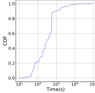
(b) The CDF of the relaying time per RESIP.
